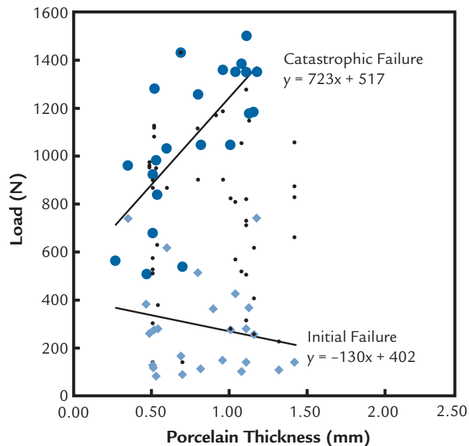
1 Plot of fracture load against porcelain veneer thickness. Initial Hertzian surface cracks are plotted as light blue diamonds; intermediate radial cracks as small black dots; and final catastrophic failures as large blue circles. Regression lines for initial Hertzian surface cracks and final catastrophic failures are plotted.
