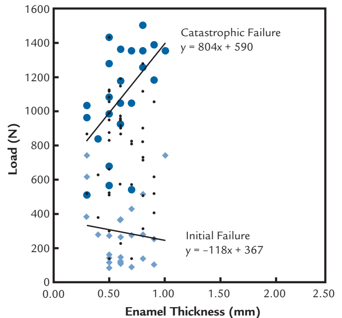
2 Plot of fracture load against supporting enamel thickness. Initial Hertzian surface cracks are plotted as light blue diamonds; intermediate radial cracks as small black dots; and final catastrophic failures as large blue circles. Regression lines for initial Hertzian surface cracks and final catastrophic failures are plotted.
