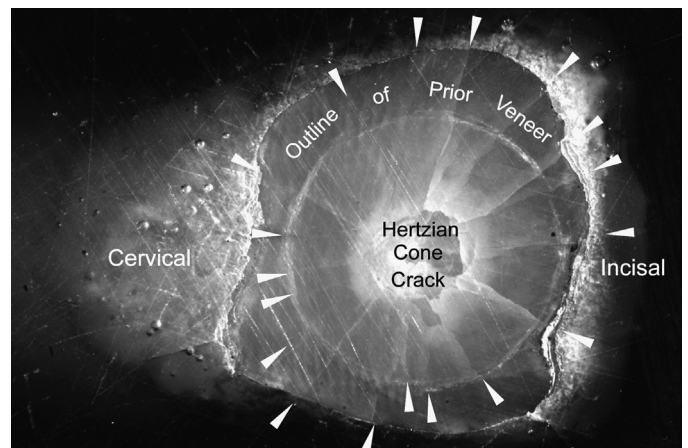
5 Facial view of transilluminated tooth after catastrophic failure and total loss of veneer; Hertzian cone crack and radial cracks (white arrows) extend through enamel.
